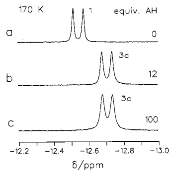
Figure 6. Hydride region of the 500-MHz ^1\text{H} NMR spectra of \text{CpRu}(\text{CO})(\text{PCy}_3)\text{H} ( 1 ) at 170 K in \text{CDCIF}_2/\text{CDF}_3 (2:1) (a) without proton donor, (b) in the presence of 12 equiv. of 2c , (c) in the presence of 100 equiv. of 2c
