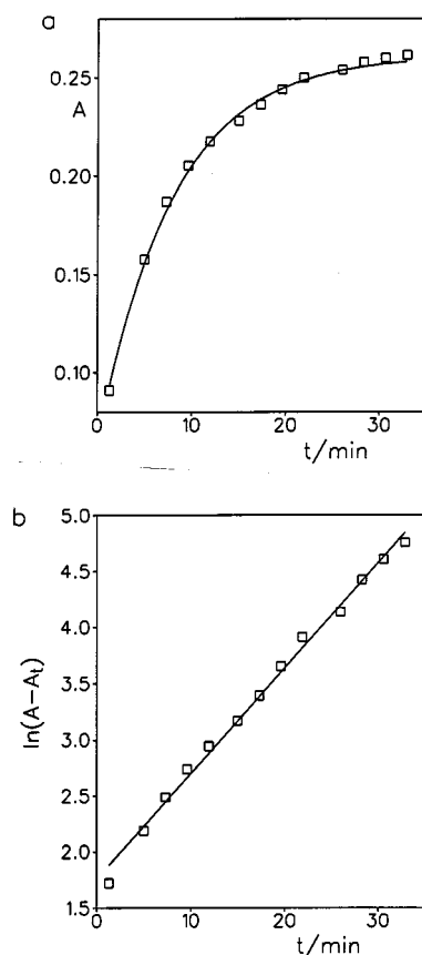
Figure 5. Kinetic curve (a) and its first-order logarithmic plot (b) for the reaction of \text{CpRu}(\text{CO})(\text{PCy}_3)\text{H} ( 1 ) (0.004 mol/L) with 8 equiv. of (\text{CF}_3)_3\text{COH} ( 2c ) in \text{CH}_2\text{Cl}_2 at 200 K
