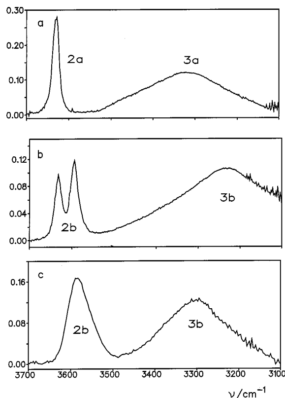
Figure 1. Room-temperature \nu_{\text{OH}} stretching bands of proton donors (0.02 mol/L) in the presence of a 2.5-fold excess of \text{CpRu(CO)(PCy}_3\text{)H} ( 1 ): (a) \text{CF}_3\text{CH}_2\text{OH} ( 2a ), hexane; (b) (\text{CF}_3)_2\text{CHOH} ( 2b ), hexane; (c) (\text{CF}_3)_2\text{CHOH} ( 2b ), \text{CH}_2\text{Cl}_2
