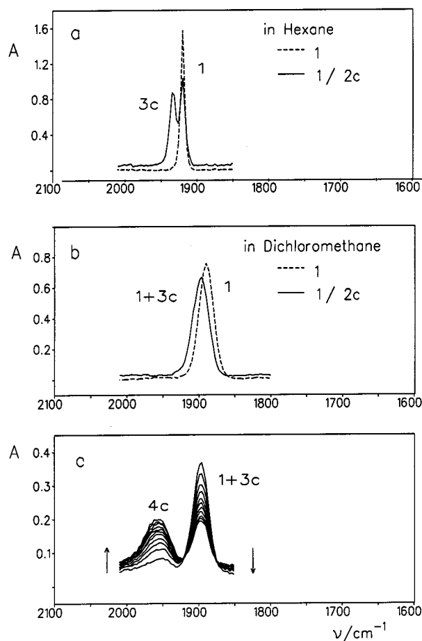
Figure 2. IR spectra in the \nu_{\text{CO}} range of CpRu(CO)(PCy 3 )H ( 1 ) (0.005 mol/L) at 200 K in hexane (a) and CH 2 Cl 2 (b, c) without proton donor (---) and in the presence of 4 equiv. of (CF 3 ) 3 COH ( 2c ) (—); (c) time-dependent changes of the sample 1/2c over a period of 30 min
