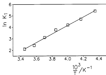
Figure 4. Van't Hoff plot of the hydrogen bonding of CpRu(CO)(P-Cy 3 )H ( 1 ) (0.005 mol/L) in the presence of 4 equiv. of 2c in hexane
