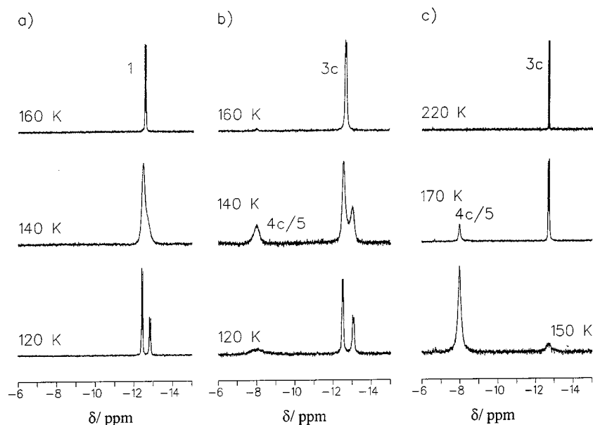
Figure 7. Hydride region of the 500-MHz ^1\text{H} NMR spectra of \text{CpRu}(\text{CO})(\text{PCy}_3)\text{H} ( 1 ) at different temperatures in \text{CDClF}_2/\text{CDF}_3 (2:1) (a) without proton donor, (b) in the presence of 12 equiv. of 2c , (c) in the presence of 100 equiv. of 2c
