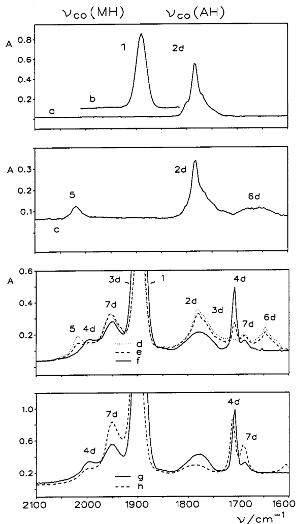
Figure 3. IR spectra of \text{CpRu}(\text{CO})(\text{PCy}_3)\text{H} ( 1 ) [ 0.001\text{ mol/L} (c), 0.01\text{ mol/L} (d–f), 0.03\text{ mol/L} (g, h)] in the presence of excess \text{CF}_3\text{COOH} ( 2d ) and a deficiency in \text{CH}_2\text{Cl}_2 ; ratio \text{1/2d} = 1:5 (c), 1:1.5 (d), 1:1 (e), 3:2 (f), 3:1 (g, h); reference spectra of 1 ( 0.01\text{ mol/L} ) and of 2d ( 0.01\text{ mol/L} ) are given in b and a, respectively; temperature 200\text{ K} (a–g), 260\text{ K} (h)
